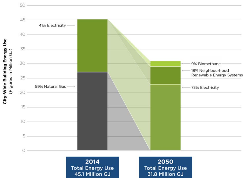
Figure 6 – City-wide Building Energy Demand Reduction 2010-2050
